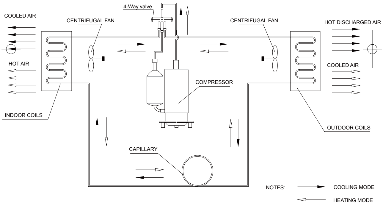
REFRIGERANT FLOW DIRECTION (рис. 2.2)
